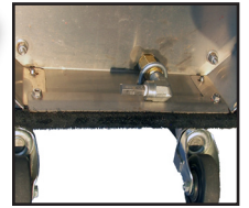
The under-deck spot remover uses a "six-shooter" nozzle to blast away gum or paint.
